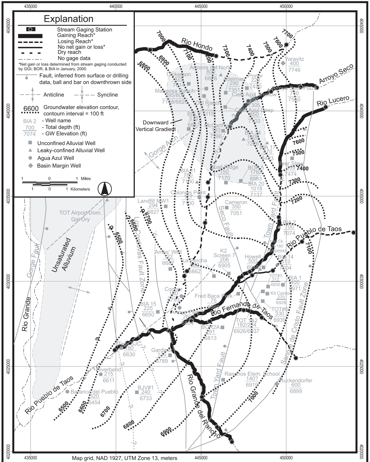
Figure 5. Shallow aquifer potentiometric surface map, gaing and losing stream reaches.
